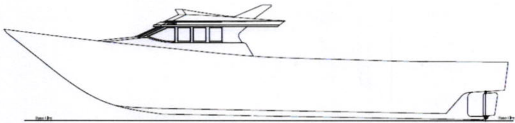
PORT SIDE PROFILE
